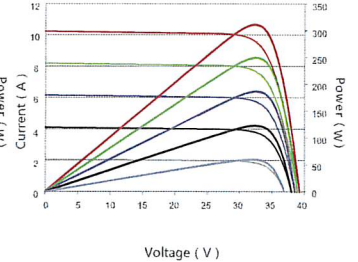
Flash Test Mode Tested by Source Simulator (310W)
