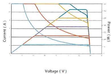
MPPT Mode Simulated Real Behavior (310W)
