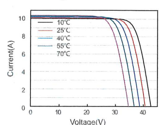
Current-Voltage Curve JAM60S12-320/PR
